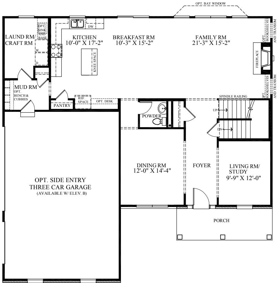
FIRST FLOOR
