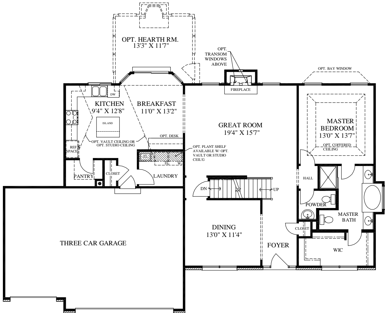
FIRST FLOOR
